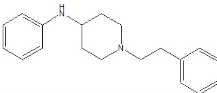
N-phenyl-1-(2-phenylethyl)piperidin-4-amine
