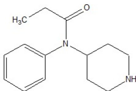
N-phenyl-N-(piperidin-4-yl)propanamide
