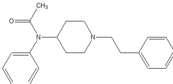
N-phenyl-N-(1-(2-phenylethyl)piperidin-4-yl)acetamide
