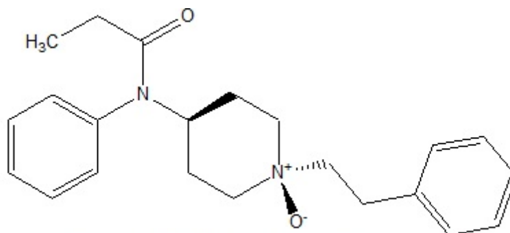
cis-trans-1-(2-Phenylethyl)-4-(phenylpropanoylamino)piperidine-1-oxide
